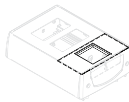
SW-IDB-S45I Power plate insert w/ 45mm openings
